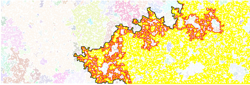
Fig. 12. Site percolation model on a square lattice in \mathbb{H} . The fixed boundary condition is enforced at the lower boundary such that on the negative real half-line all the sites are unoccupied, while on the other half-line the sites are occupied. This imposes an interface (the perimeter in red) at the boundary of the spanning cluster (yellow colored) starting from the origin and ending at the upper boundary (the interface is defined uniquely by using the turn-right tie-breaking rule [269]). The external perimeter is shown by the dark solid line. In the scaling limit, as the lattice constant goes to 0, the perimeter and external perimeter then converge in distribution to SLE_6 and SLE_{8/3} , respectively. (For interpretation of the references to color in this figure legend, the reader is referred to the web version of this article.)
