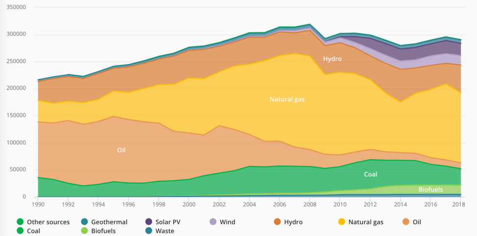
Electricity generation by source, Italy 1990-2018 GWh
