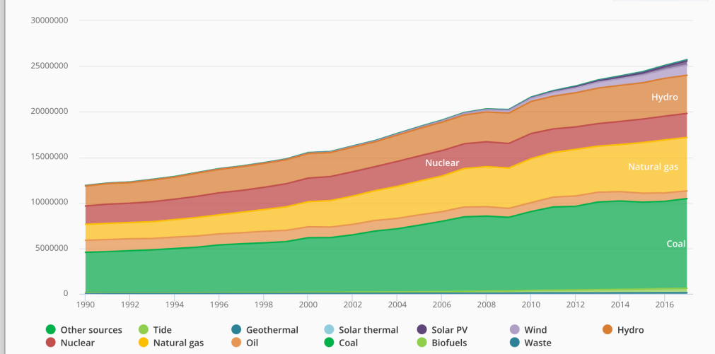
Electricity generation by source, World 1990-2017 GWh
